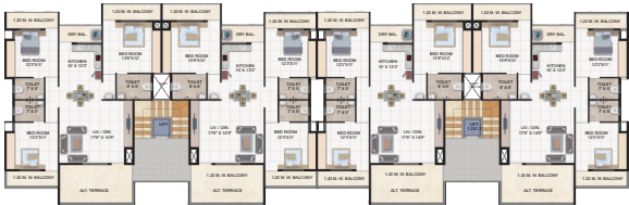
FIRST & THIRD FLOOR PLAN
